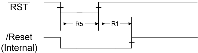
Figure 24-7. External Reset Timing ( \overline{RST} )
